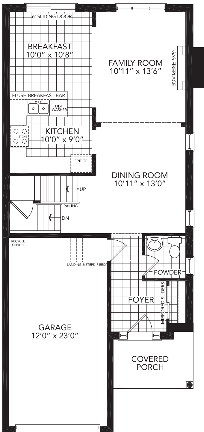
GROUND FLOOR ELEVATION 'A' & 'C'
