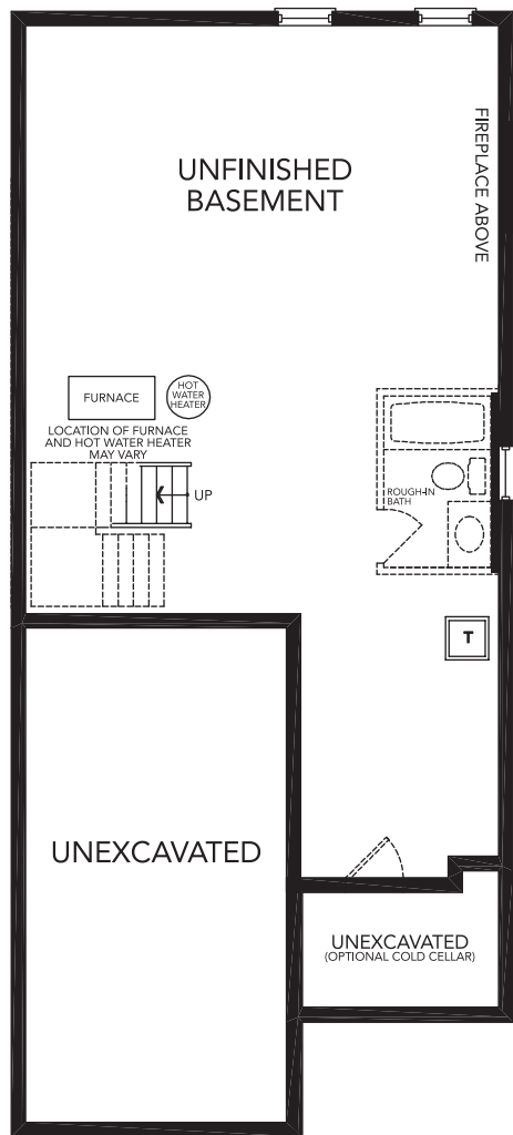
BASEMENT FLOOR ELEVATION 'A' & 'C'
