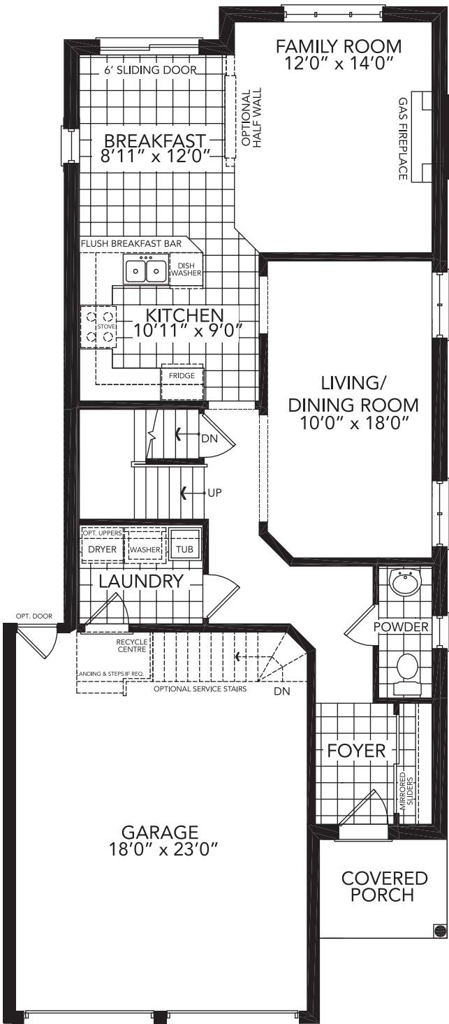
GROUND FLOOR ELEVATION 'A' & 'C'
