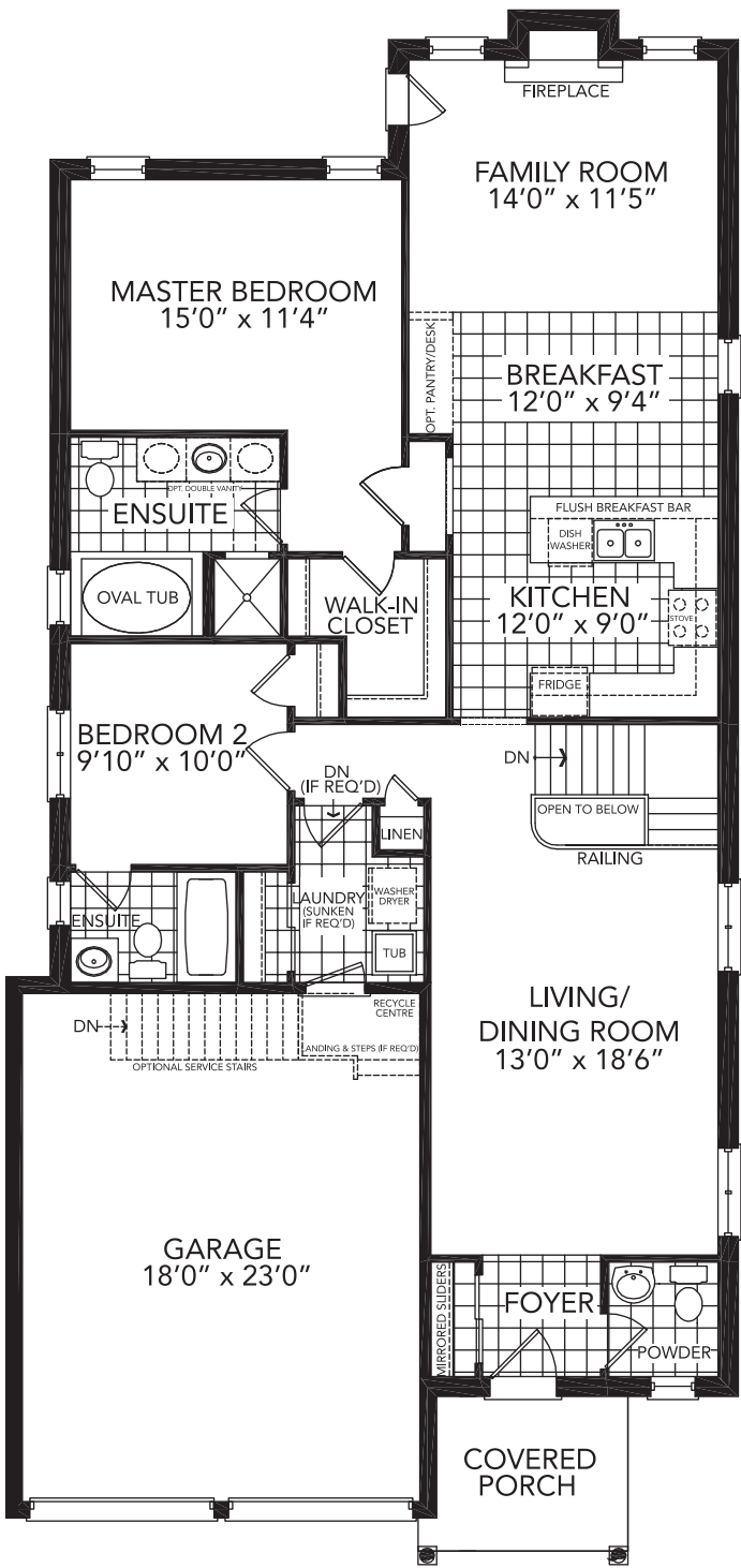
GROUND FLOOR ELEVATION 'A'
