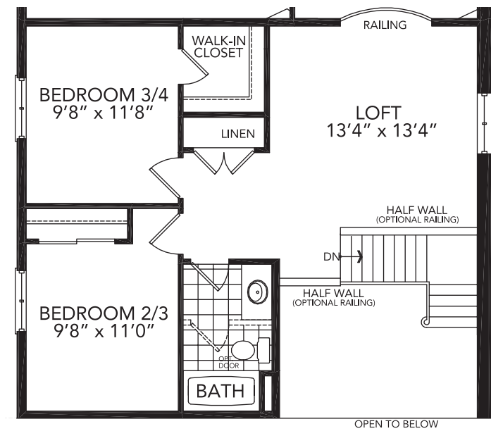
LOFT FLOOR ELEVATION 'C' & 'D'
