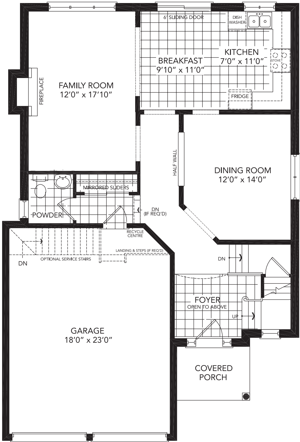
GROUND FLOOR ELEVATION 'A' AND 'B'
